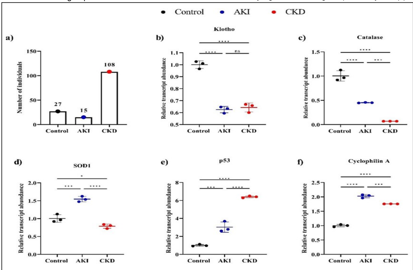
Figure 1: Relative transcript abundance of KL , CAT , SOD1 , p53 and CyPA genes
