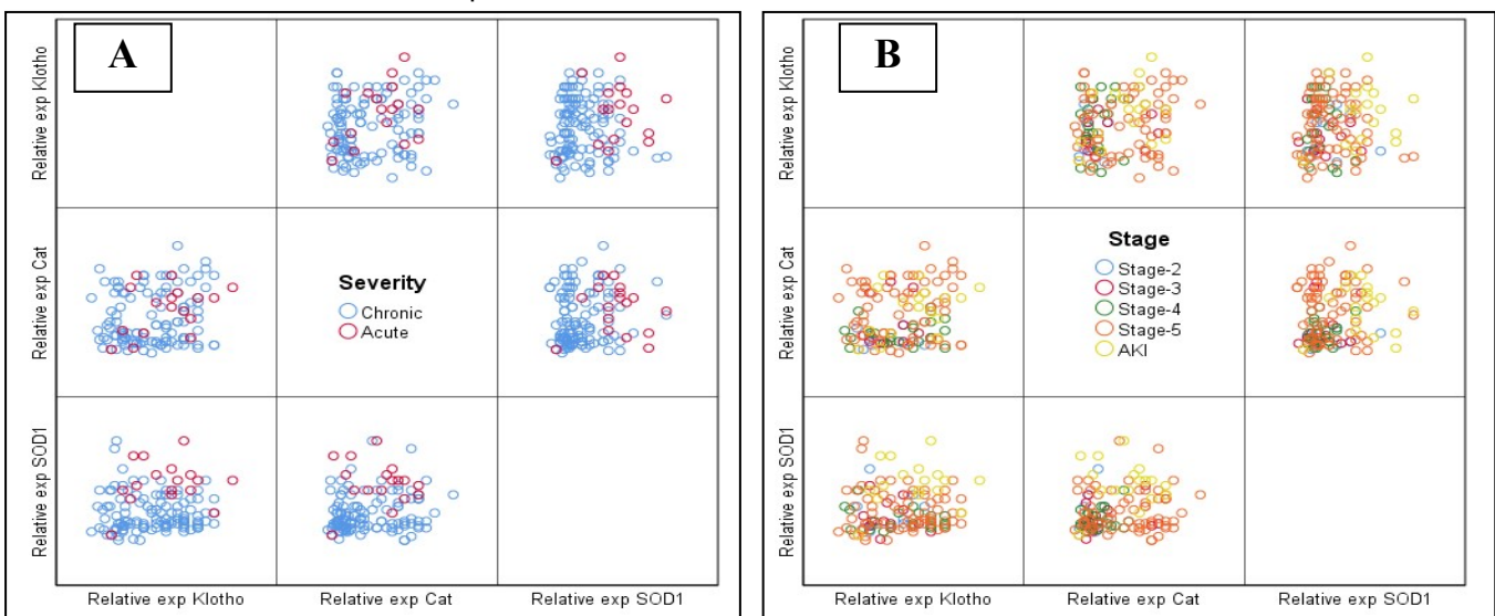
Figure 3: Correlation of KL, CAT, and SOD1 genes in relation to severity of disease among AKI and CKD (A) and CKD stages (B)
