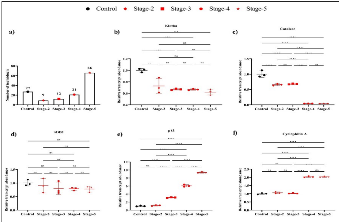
Figure 2: Relative transcript abundance of KL, CAT, SOD1, p53 and CyPA genes across CKD stages
