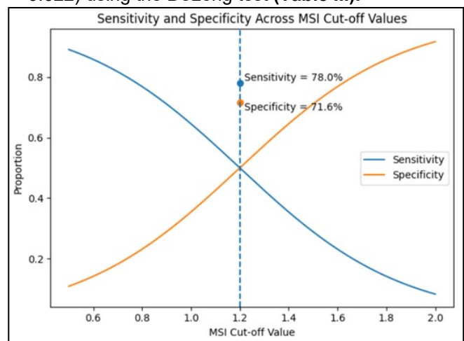
Figure 1: Sensitivity and specificity across different Modified Shock Index (MSI) cut-off values for prediction of in-hospital mortality
